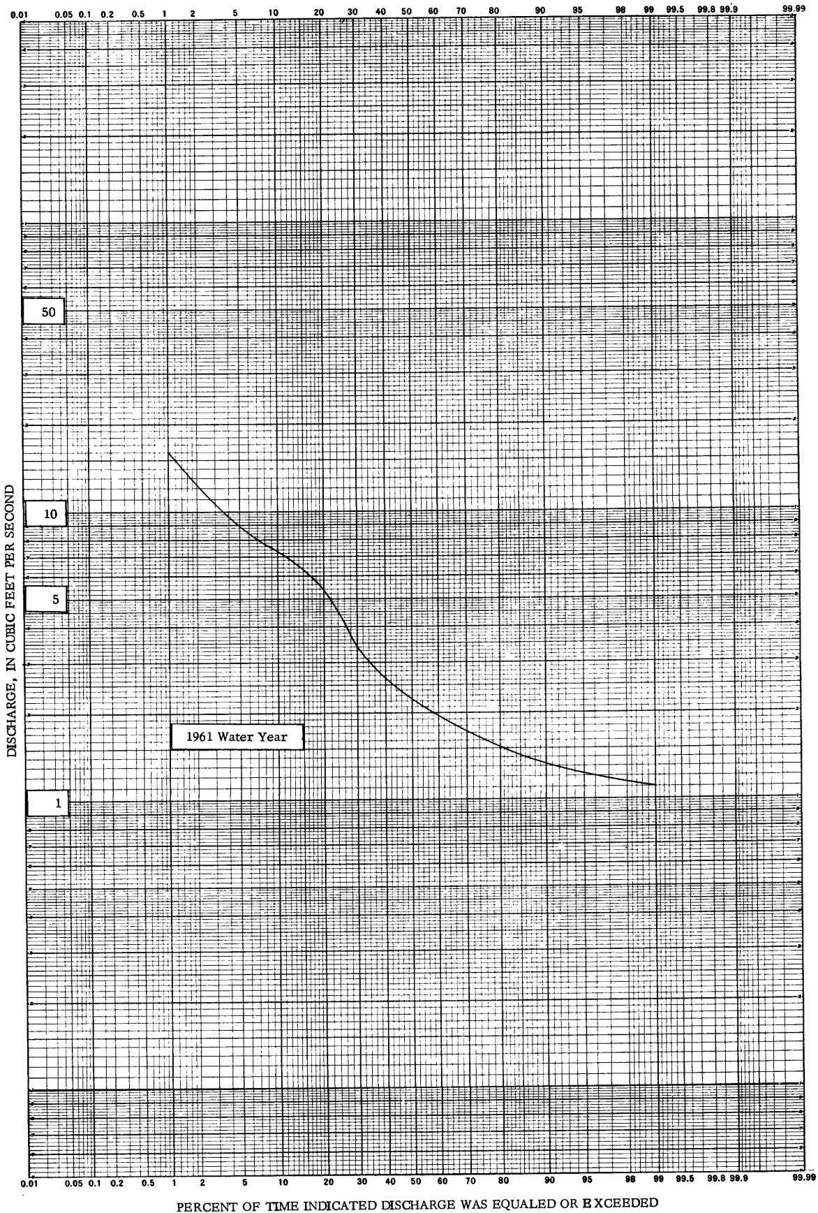
Figure 24. --Duration curve of daily flow, Saddle River near Spring Valley, N. Y.
